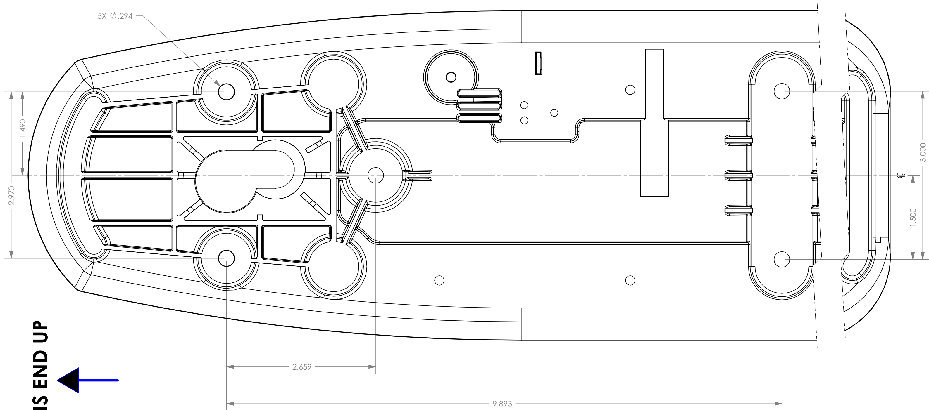
Sea Shelter™ 2 TEMPLATE: Y1-06-0247 REV A
